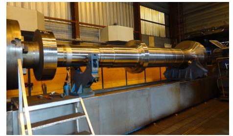
Shaft on 4G Horizontal Lathe
