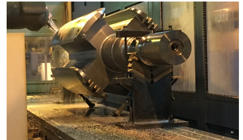
Rotor on CORREA Milling Machine
