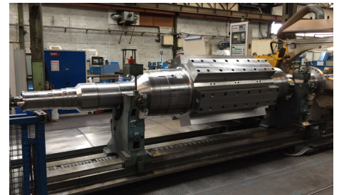
Rotor on Gioria Cylindrical Grinding Machine
