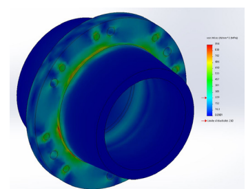
Mechanical Bonding Simulation
